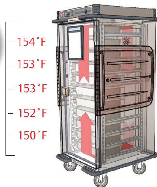
T-Series with Transport Armour®
