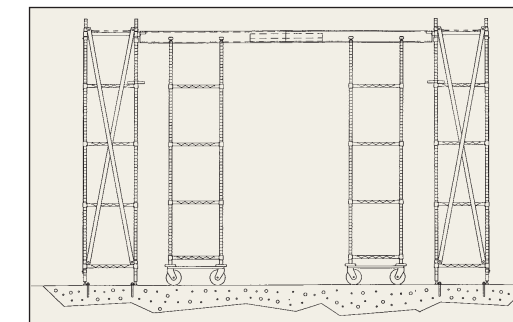
Single-Length System
