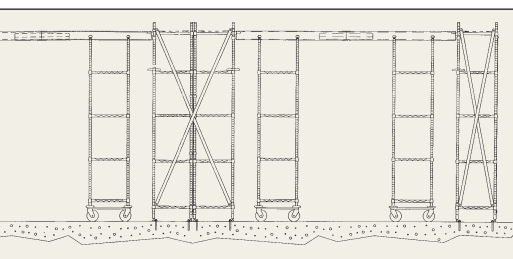
Double-Length System
